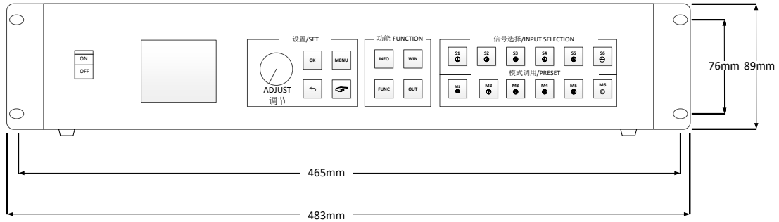
Front panel dimensions
