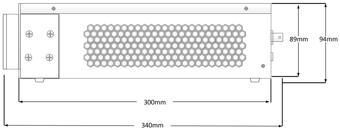
side panel dimensions
