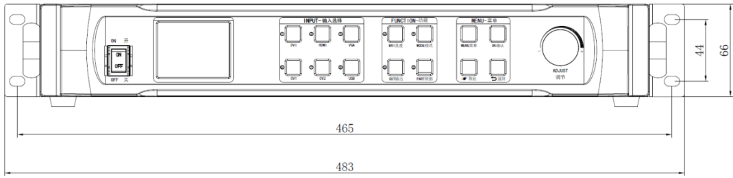
Front panel size drawing
